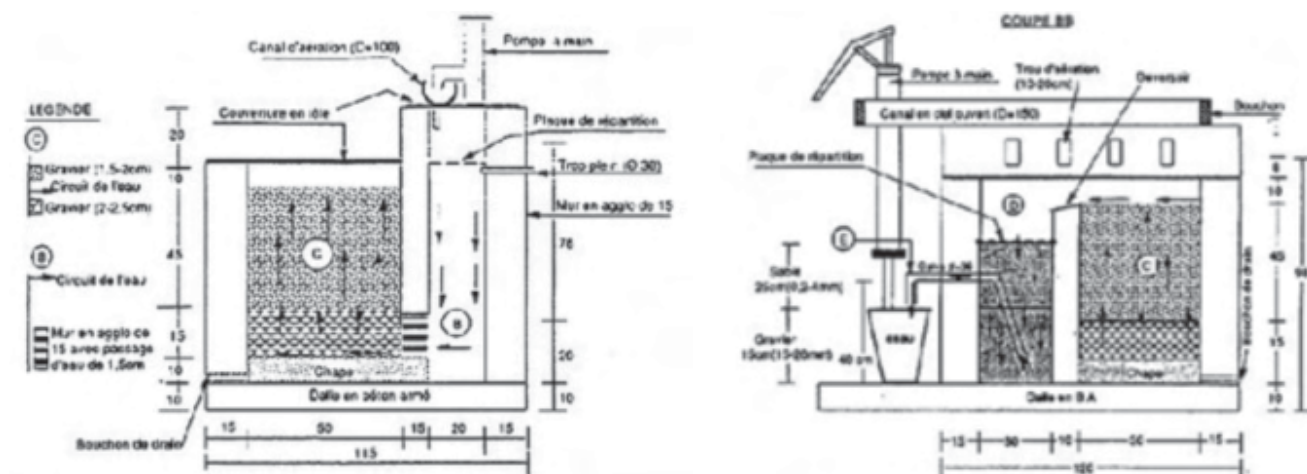
Figure 63: Schematic of a Typical Iron Removal Unit
