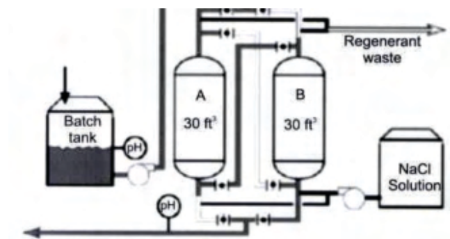
Figure 93: Schematic diagram of Lawrence Liverpool National Laboratory's hexavalent Chromium removal unit
