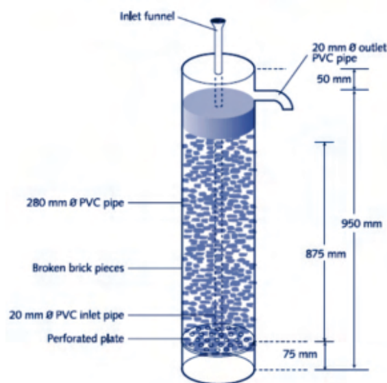
Figure 49: Domestic De-fluoridation unit using Brick Pieces
