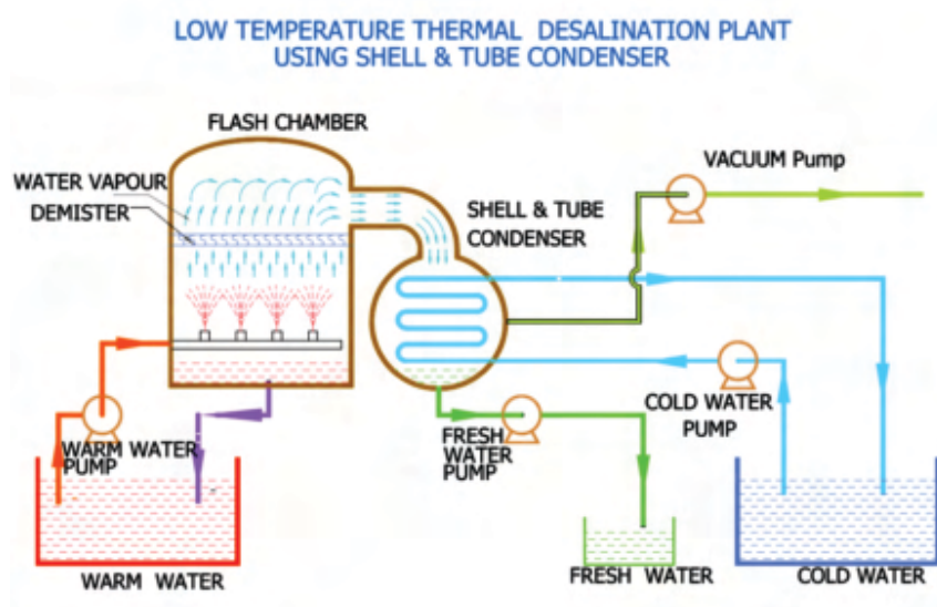
Figure 74.1: LTTD process
