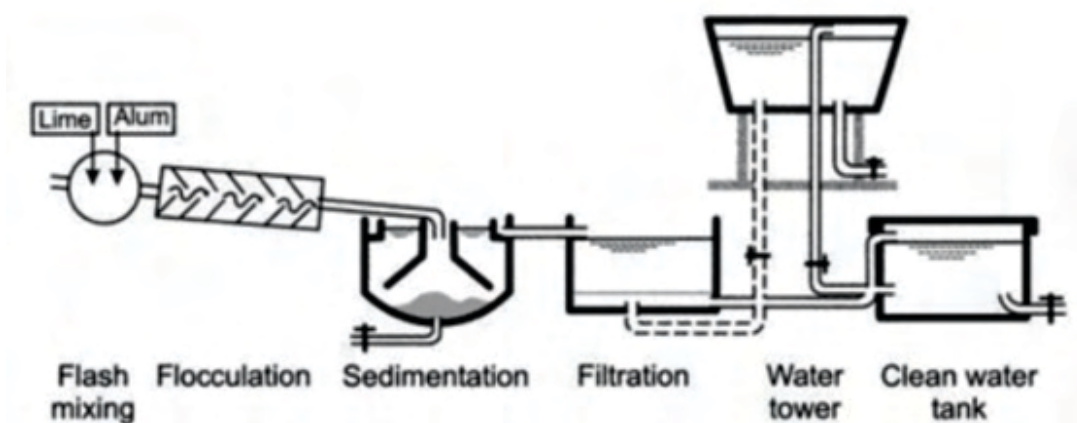
Figure 42: Fill and draw de-fluoridation plant based on Nalgonda technology
