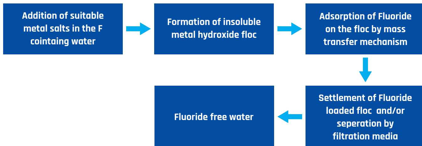
Figure 39: Steps in coagulation precipitation technique
