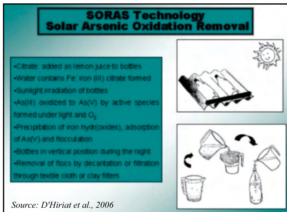
Figure 1: Solar Oxidation and Removal of Arsenic (SORAS)
