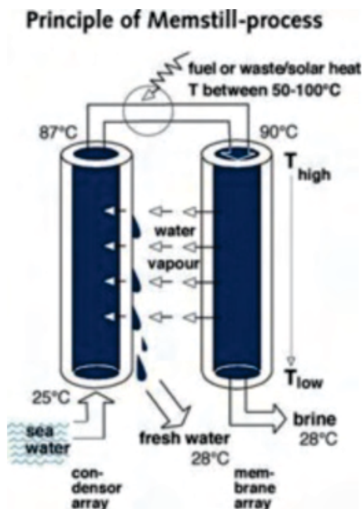
Figure 51: Memstill Technology
