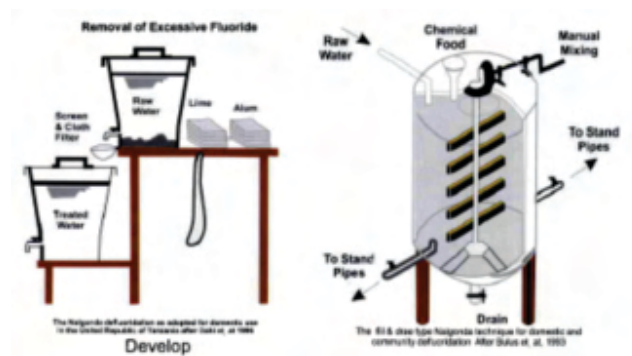
Figure 40: Configuration of Nalgonda Technology
