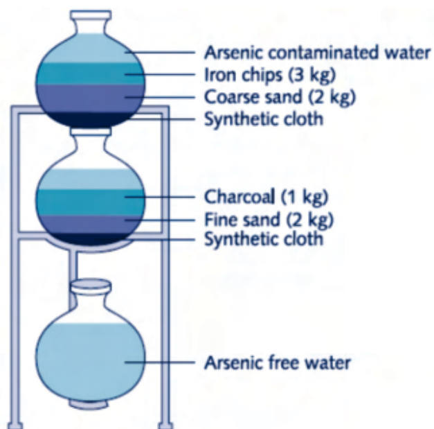
Figure 19: Three pitcher filter
