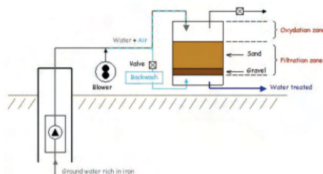
Figure 62: Schematic Diagram of Lenntech Iron Removal Plant
