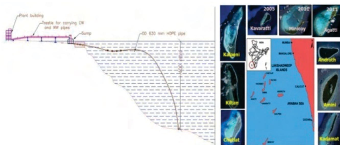
Figure 75: Layout for shore based LTTD plant (inset figure showing Lakshadweep Islands)
