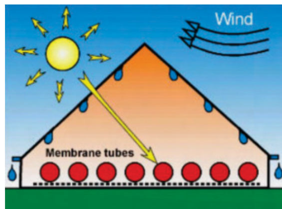
Figure 52: The Solar Dew Collector System
