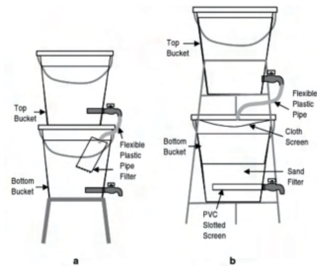
Figure 4: Double-bucket household Arsenic treatment unit
