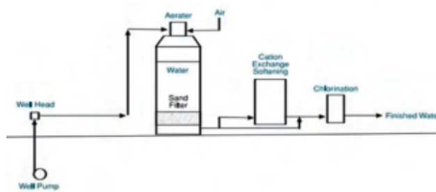
Figure 21: Aeration/Sand Filtration Unit, Cation Exchange Softening and Chlorination
