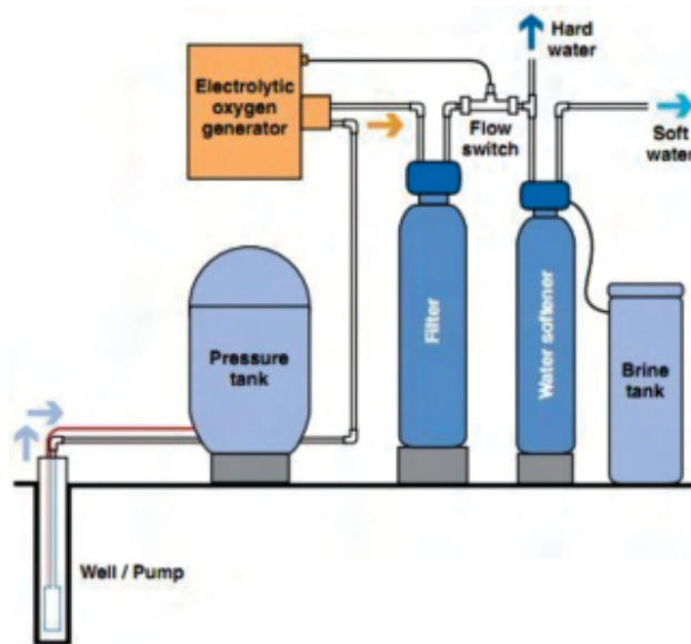
Figure 68: The WATER D.O.G. Iron Hunter HD
