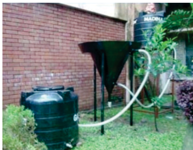
Figure 30: ARUBA Arsenic Removal Plant Prototype
