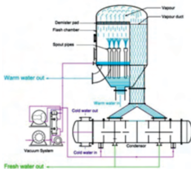
Figure 77: Process component
