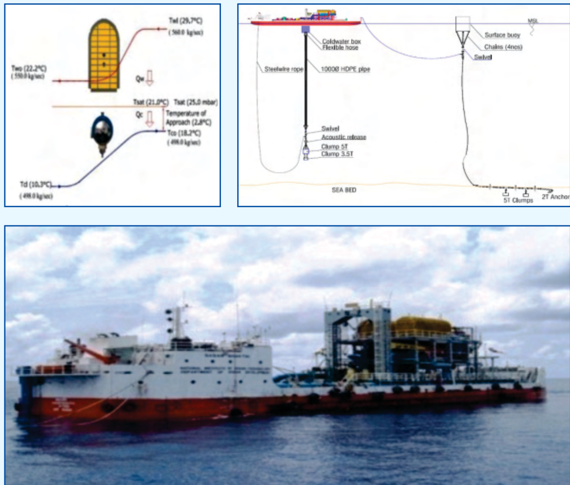
Figure 83: Details of the barge mounted 1 MLD Demonstration LTTD plant
