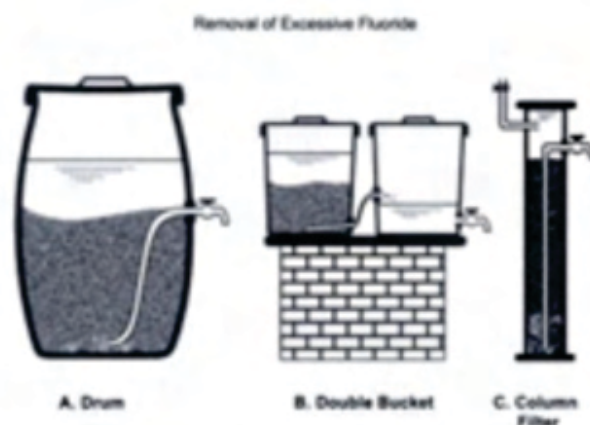
Figure 38: Common Sorption De-Fluoridation Units
