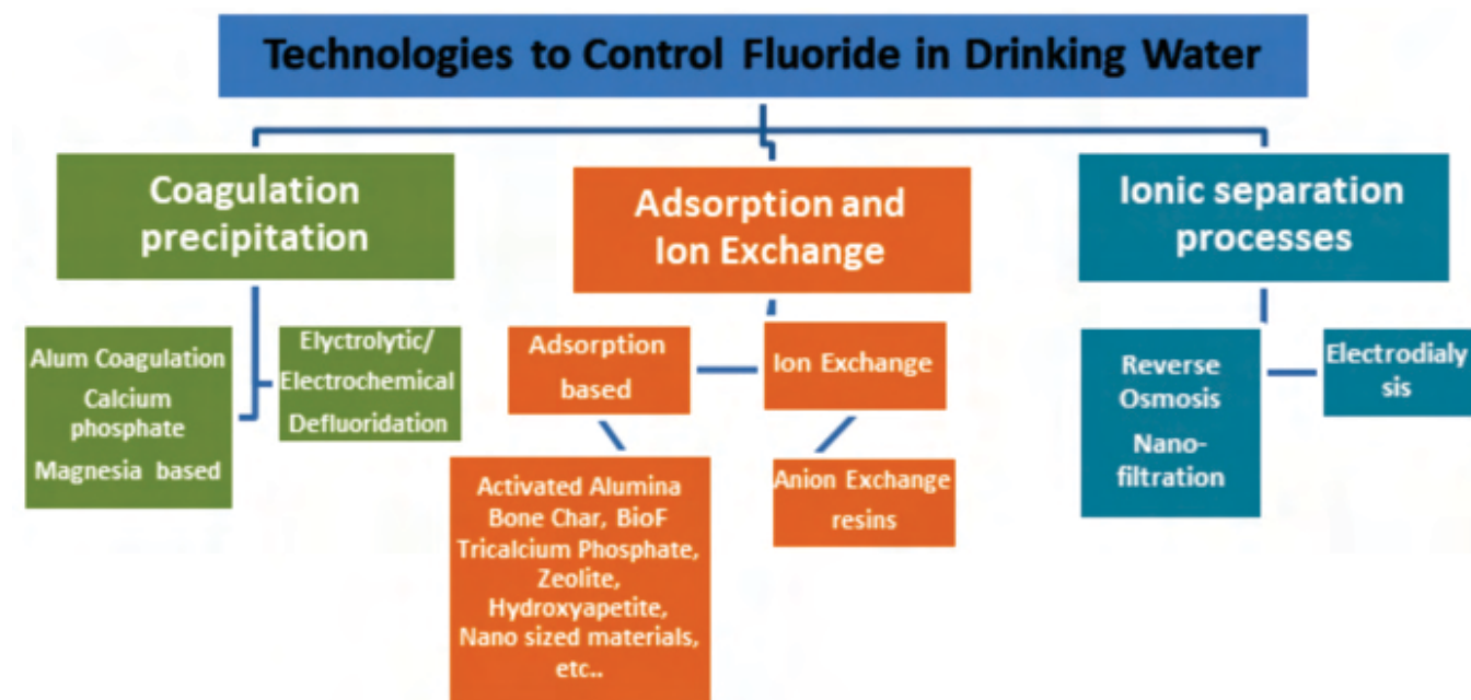
Figure 36: Defluoridation techniques
