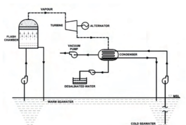
Figure 79: Schematic of OC OTEC based desalination
