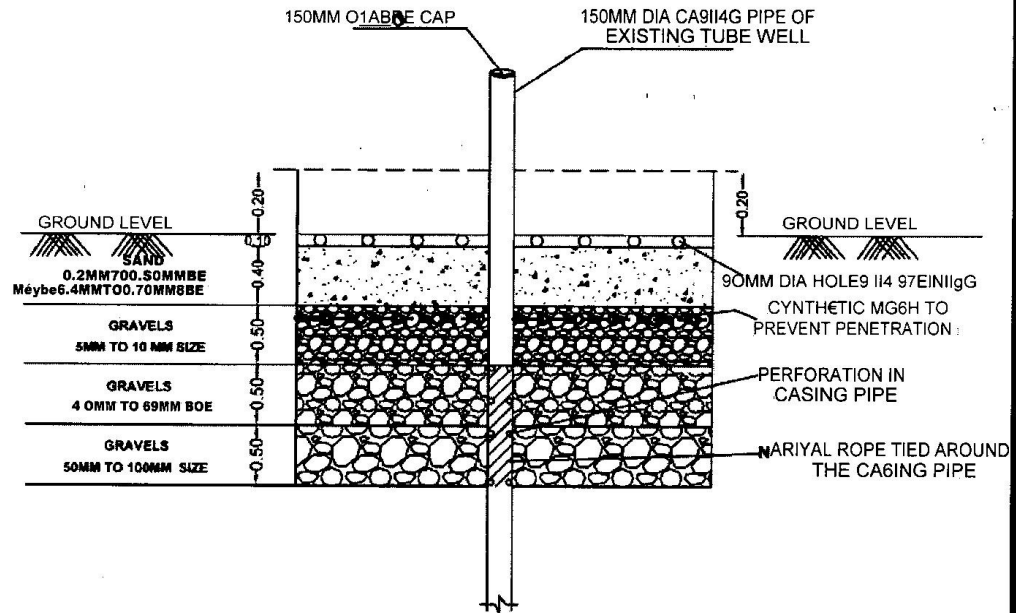
SECTIONAL ELEVATION
