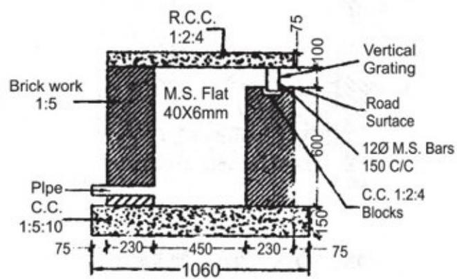
ROAD GULLEY CHAMBER 400X450X775 (VERTICAL GRATING)
