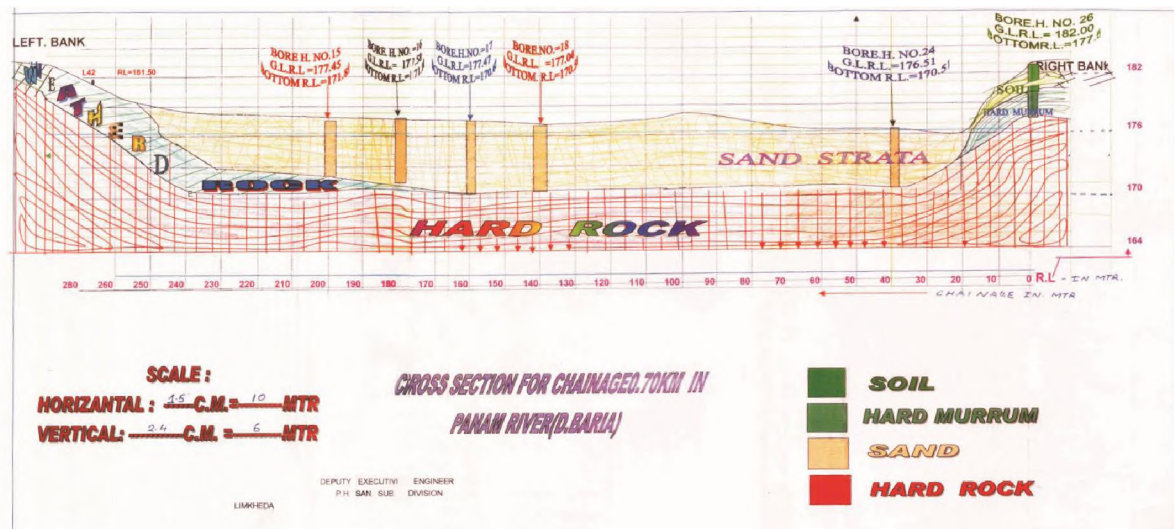
8.30 b Section showing positioning of a Sub Surface Dyke
