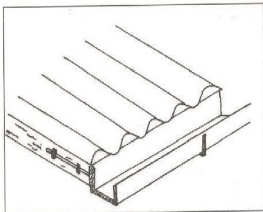
Fig. 9.2 Rectangular Gutter
