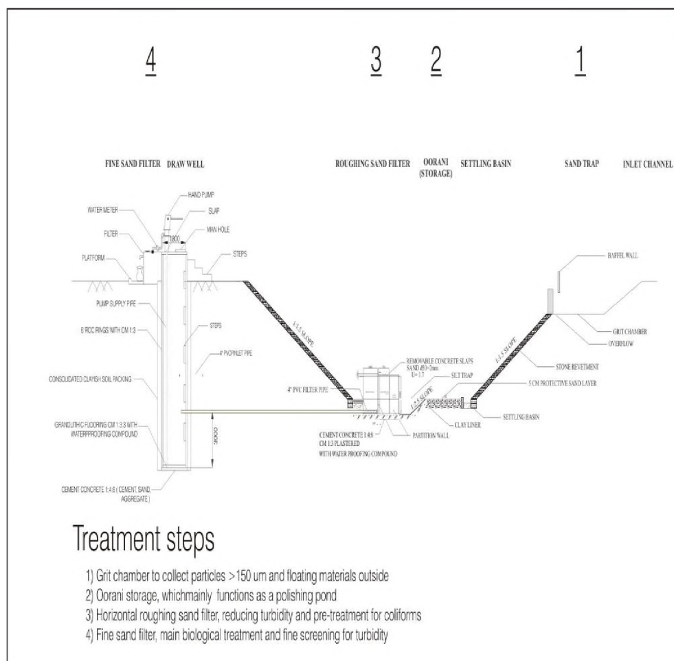
Fig 8.18 Typical Section of an Oorani
